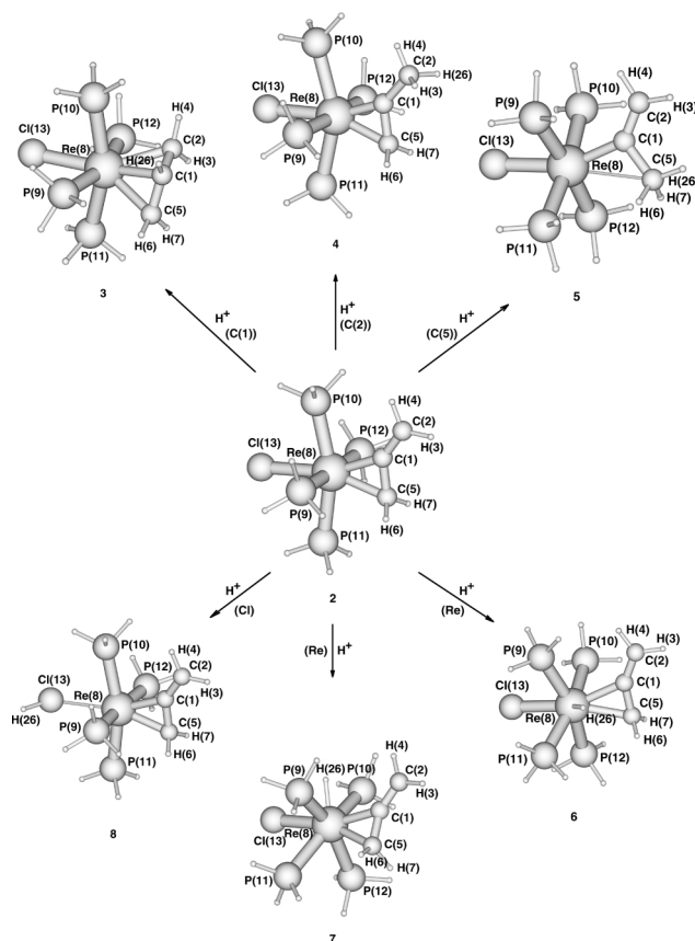
Fig. 1 Optimized structures for the allene complex 2 and for the derived monoprotinated complexes 3–8 (numbers following the order of increasing energy) ( 8 is the most favourable intermediate towards 4 ).
