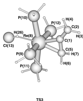
Fig. 4 The transition state for the Cl(13) \rightarrow Re proton migration.
