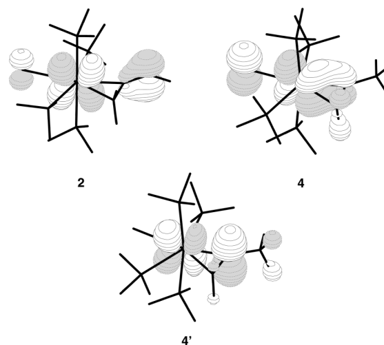
Fig. 5 The HOMOs of the allene ( 2 ), \eta^2 -vinyl ( 4 ) and reduced \eta^2 -vinyl ( 4' ) complexes.
