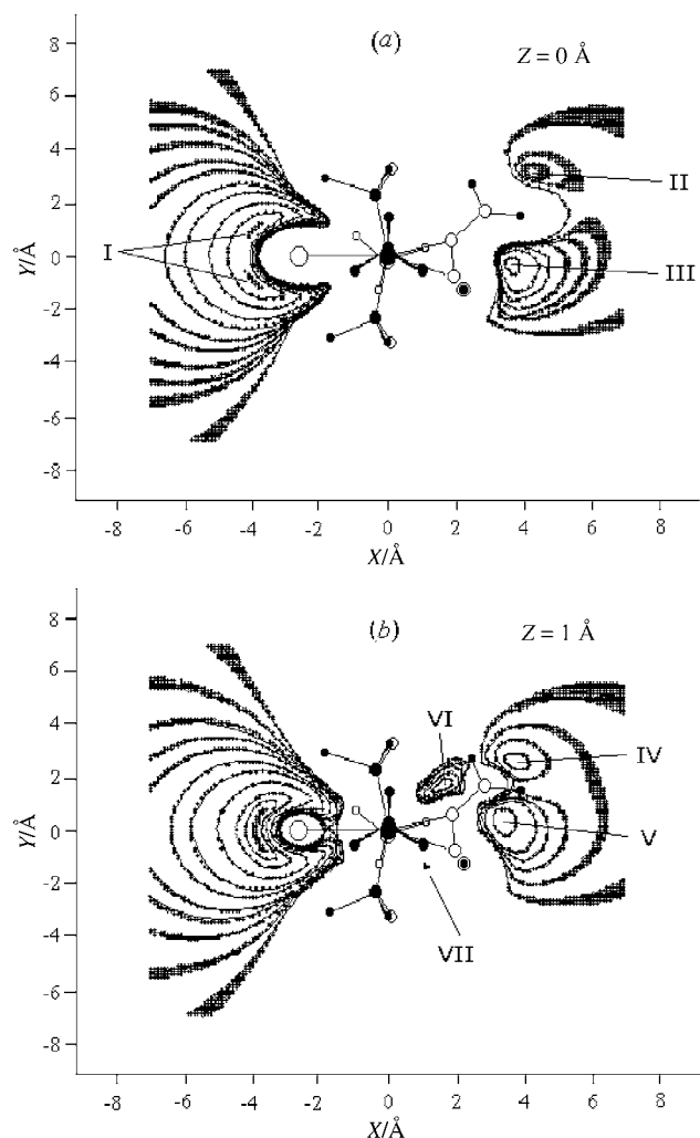
Fig. 2 Distribution of electrostatic potential for compound 2 : (a) in the plane of the allene fragment ( z = 0 Å); (b) in the parallel plane at 1 Å distance ( z = 1 Å).
